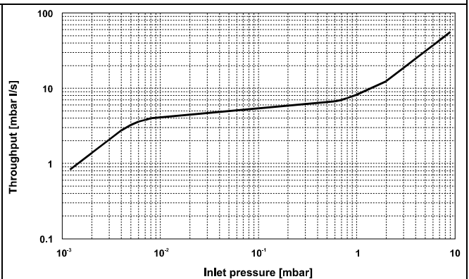
Graph of nitrogen throughput vs inlet pressure using the recommended mechanical forevacuum pump
