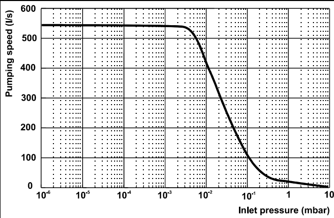
Graph of nitrogen pumping speed vs inlet pressure (with inlet screen)
