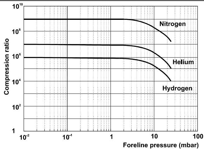
Graph of compression ratio vs foreline pressure
