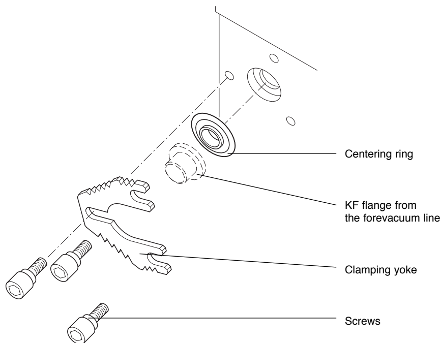
Fig. 8 Connecting the forevacuum line
