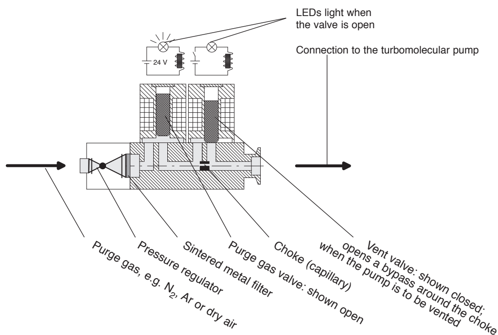
Fig. 14 Purge gas and venting valve assembly (schematic)
