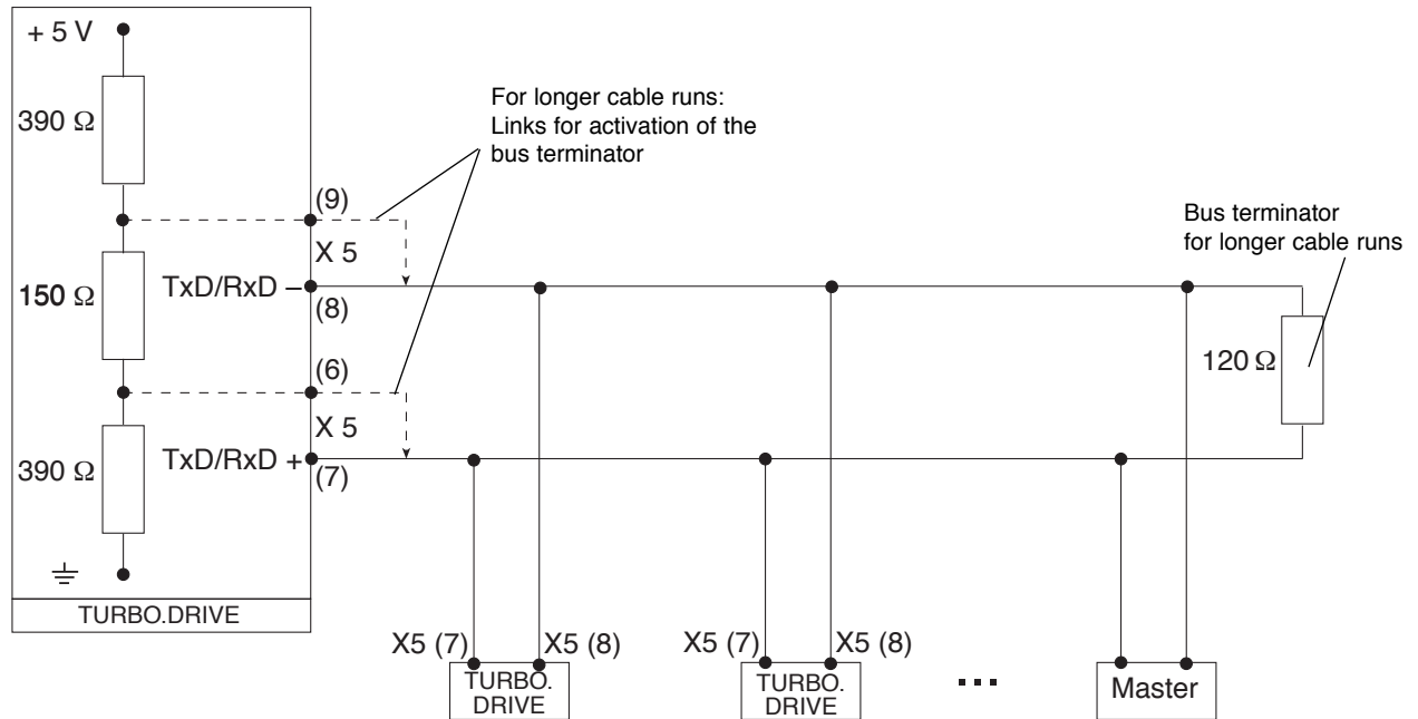
Fig. 23 Connection of the RS 485 bus
