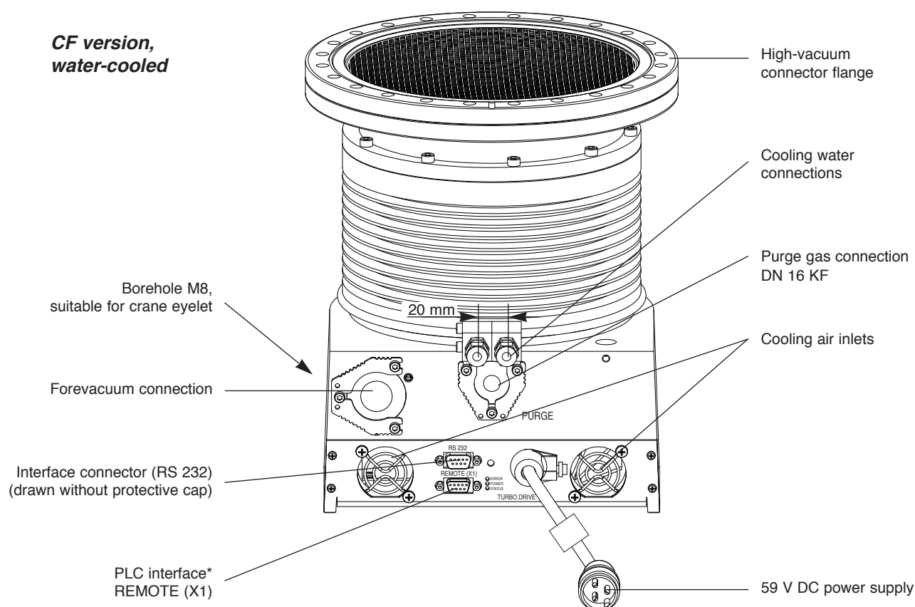
Fig. 6 Connection elements
