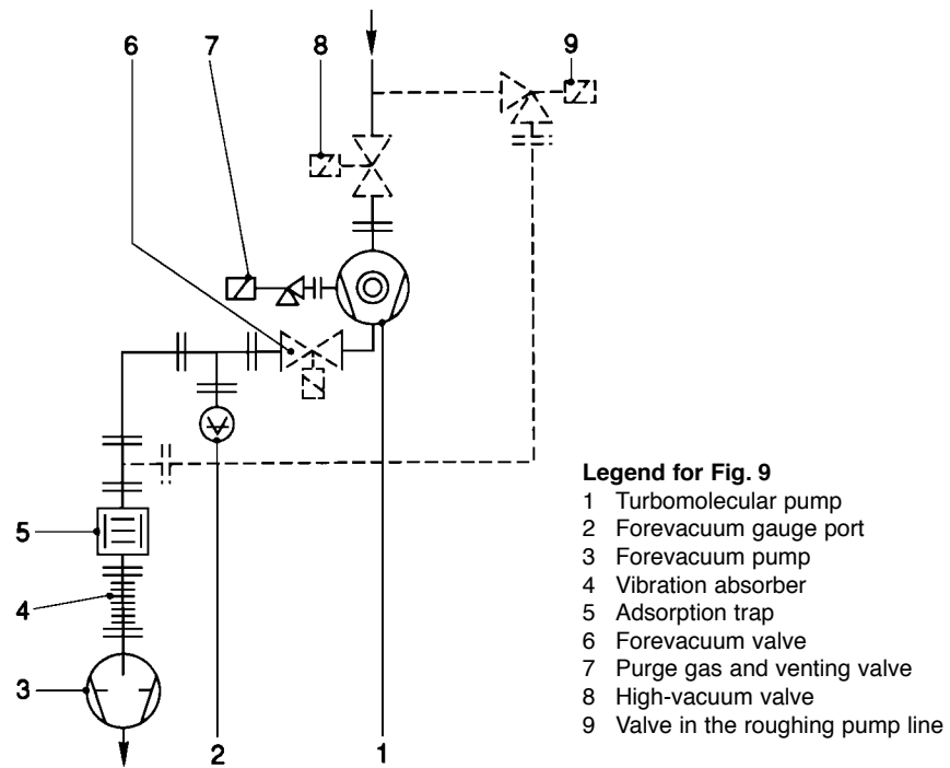
Fig. 9 Schematic of a turbomolecular pump system
