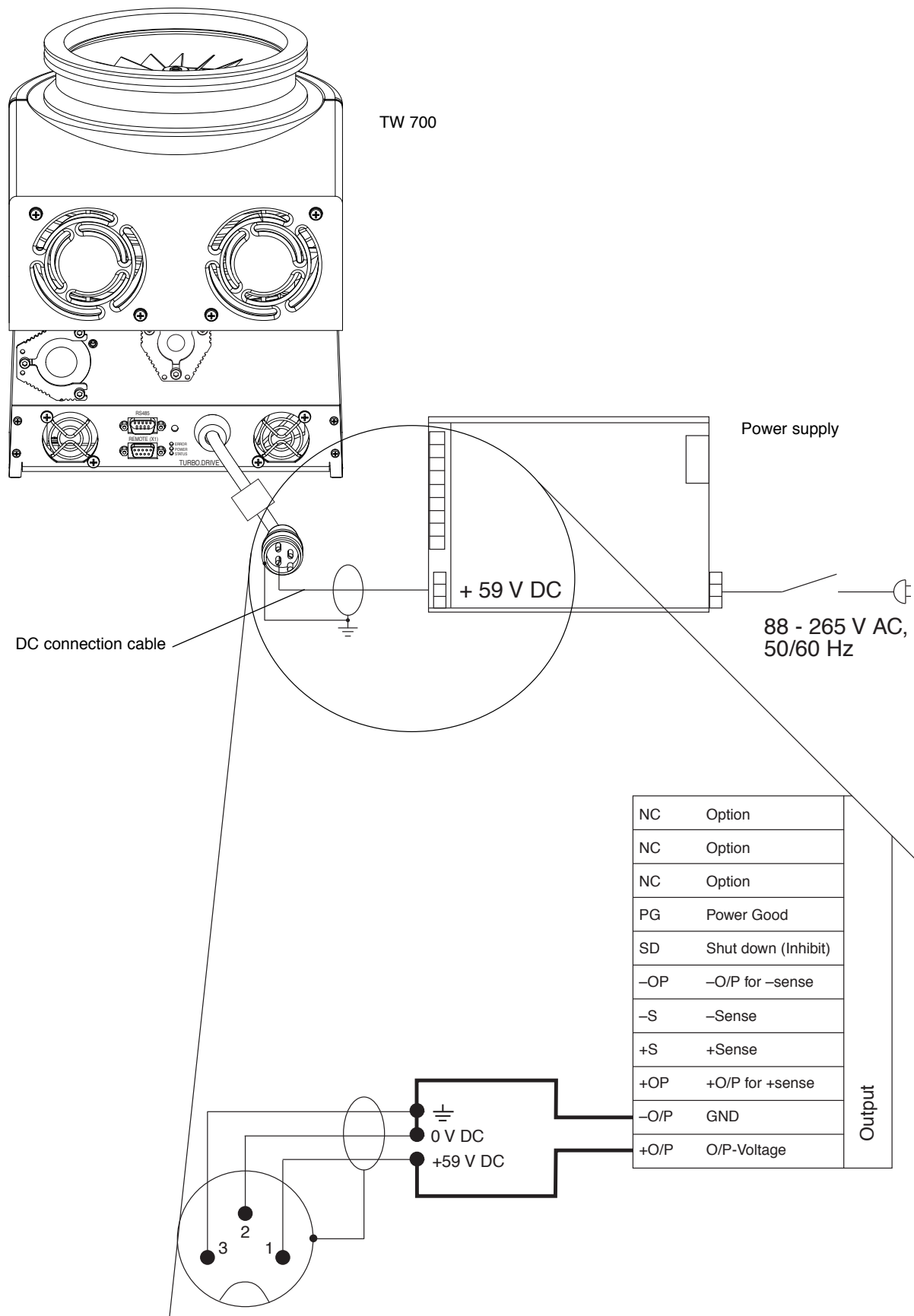
Fig. 16 Connection of the power supply
