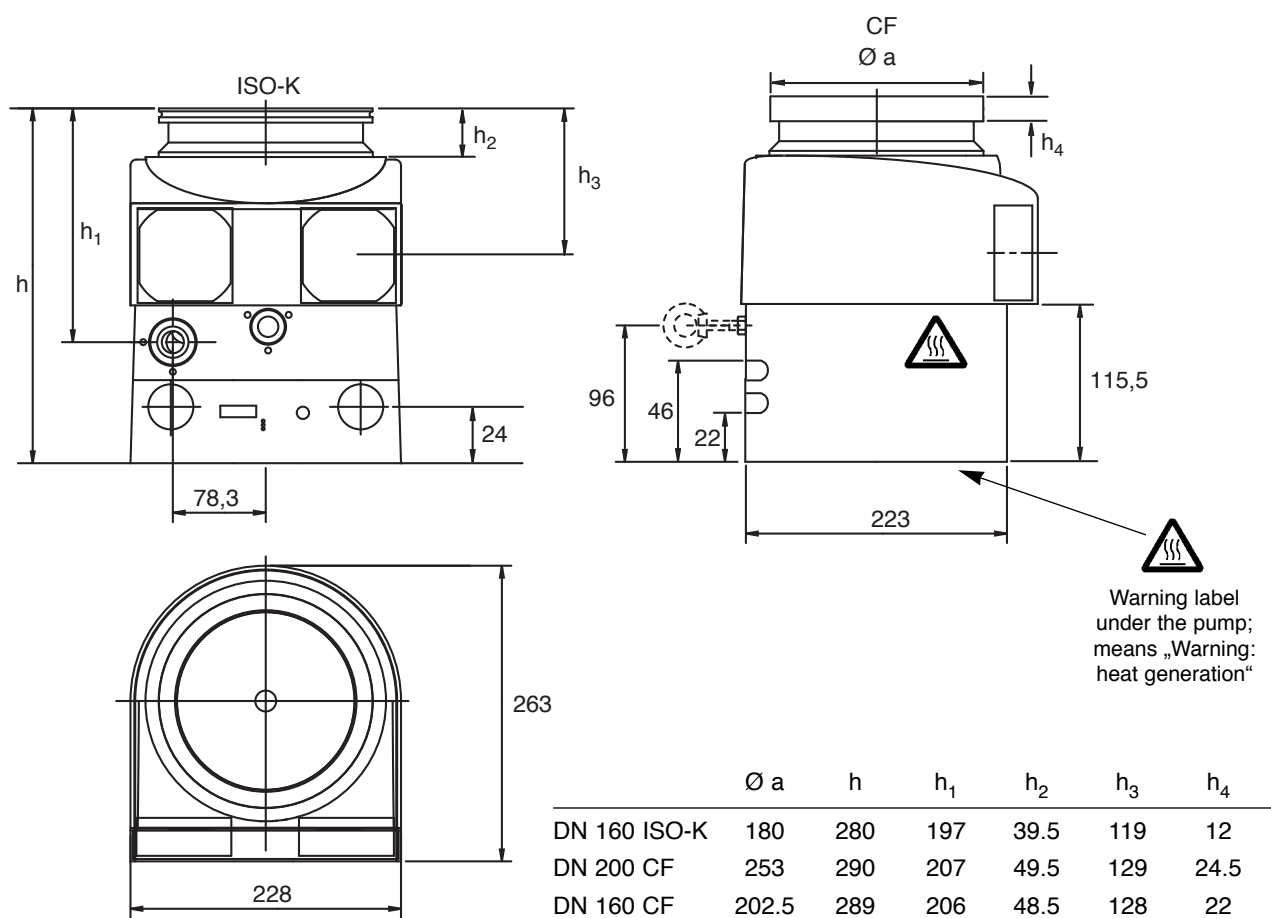
Fig. 3 Dimensional drawing, dimensions in mm
