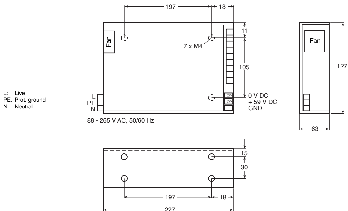
Fig. 4 Dimensional drawing of the power supply, dimensions in mm
