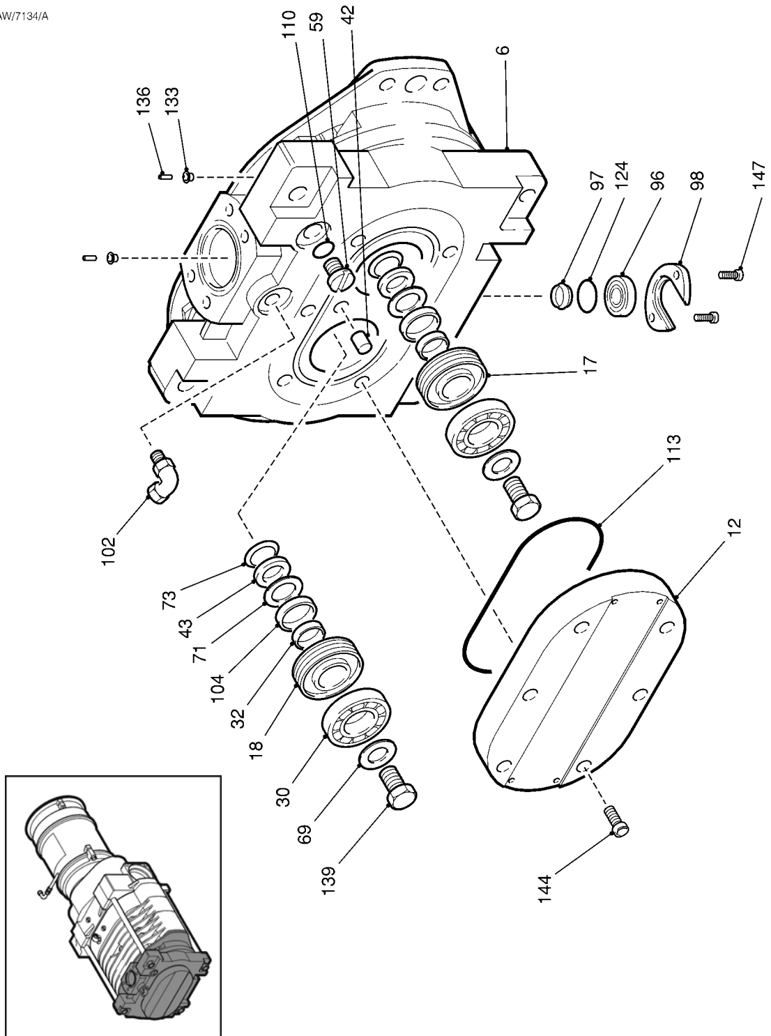
Figure 2 - QDP and iQDP HV Stator assembly
