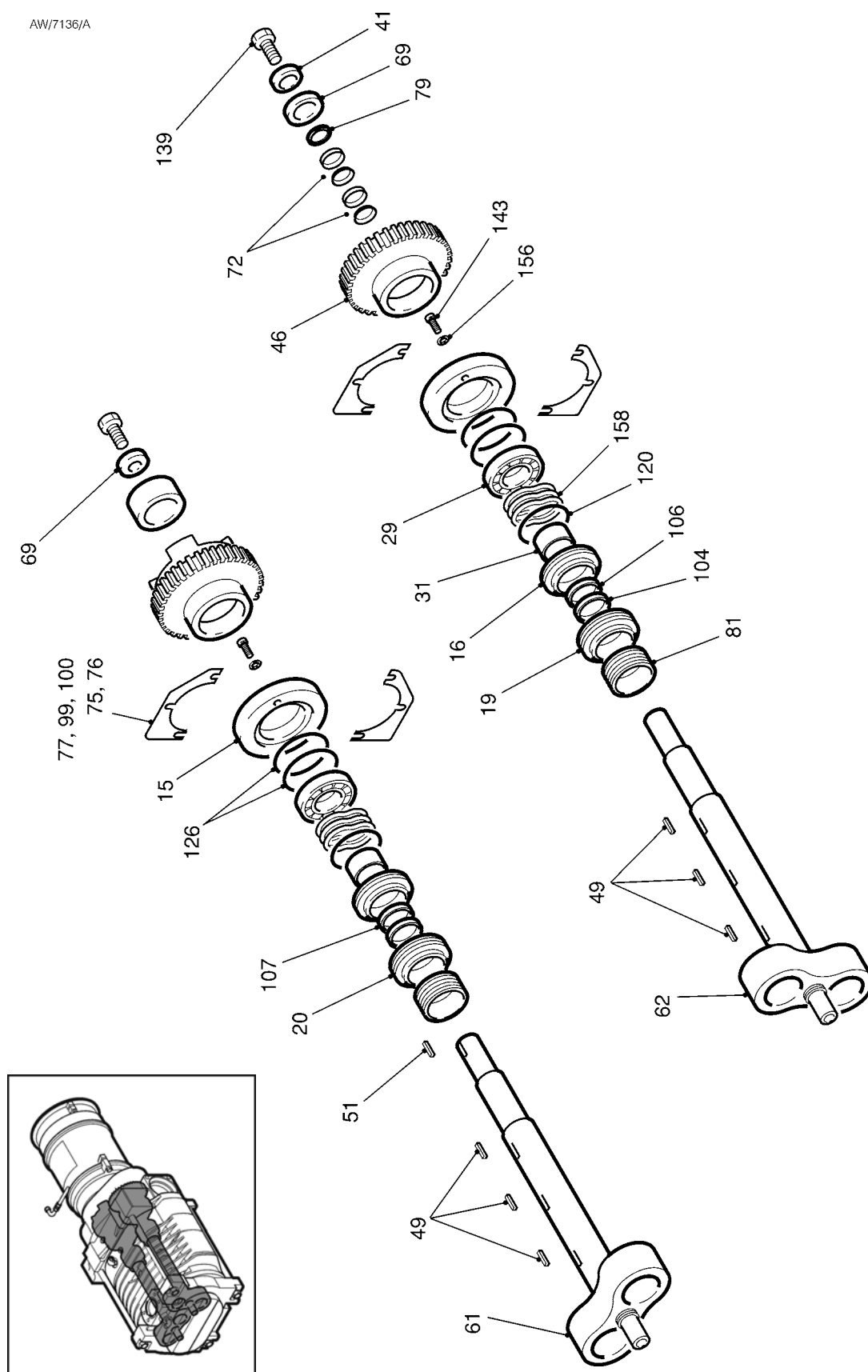
Figure 11 - QDP and iQDP80 Rotor assemblies
