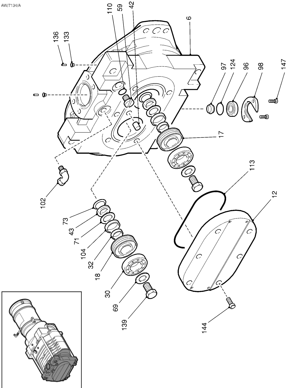
Figure 9 - QDP and iQDP80 HV Stator assembly
