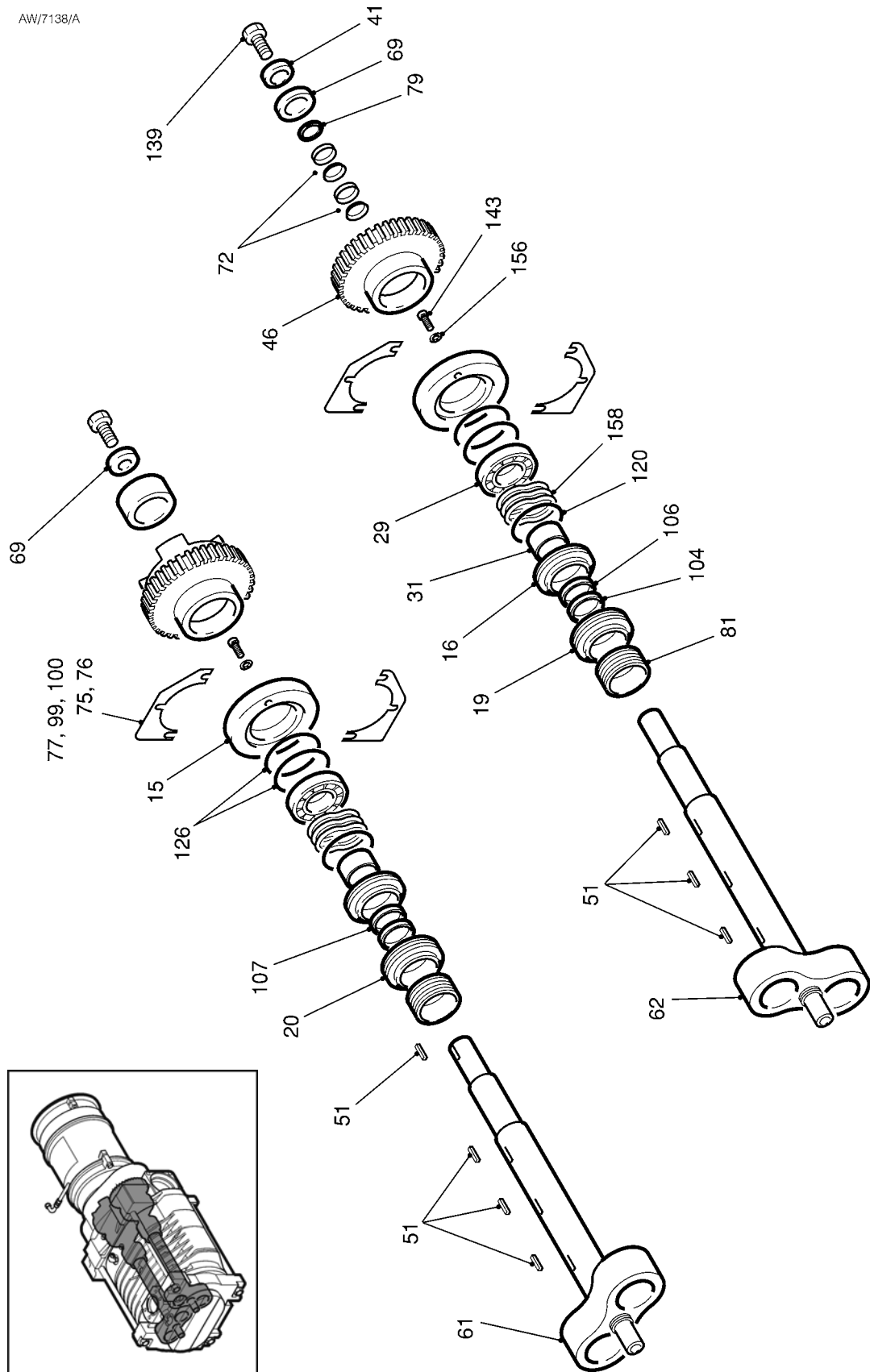
Figure 4 - QDP and iQDP40 Rotor assemblies
