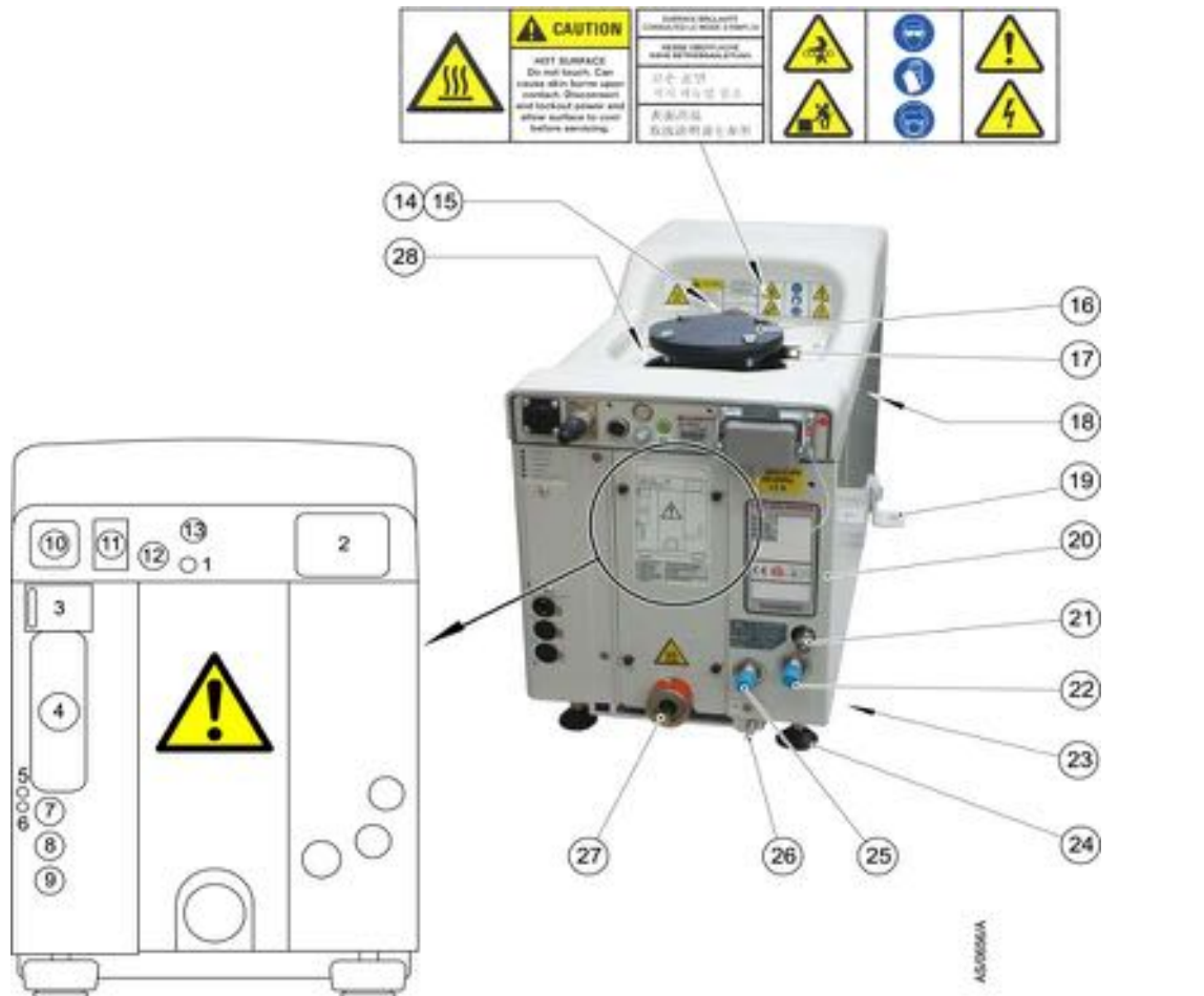
Figure 2 - The controls/connectors
