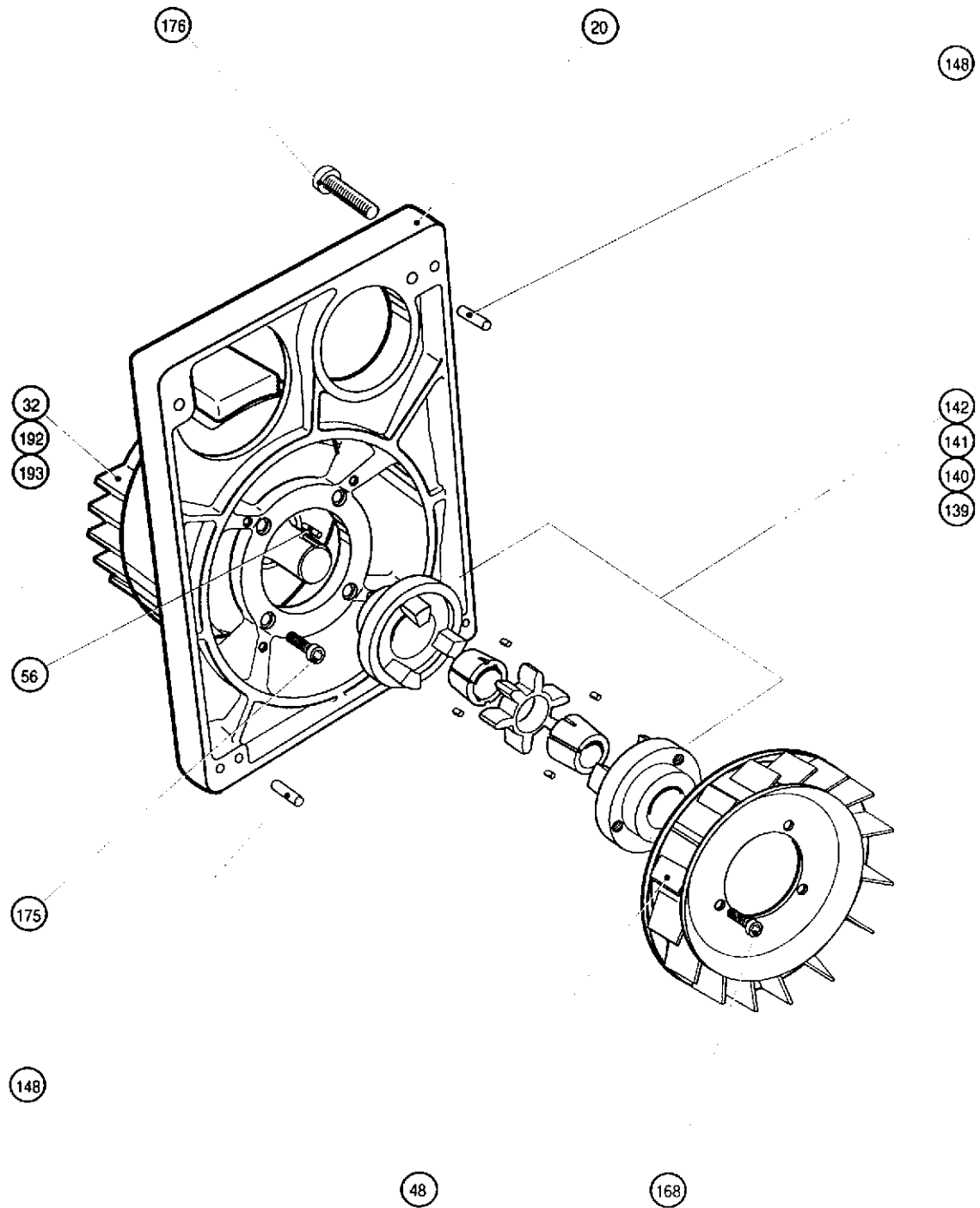
Figure 15 - (G) E2M40 Motor plate sub-assembly
