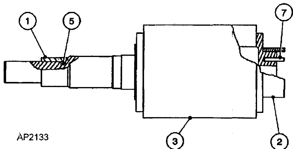
Figure 4a - HV rotor assembly
